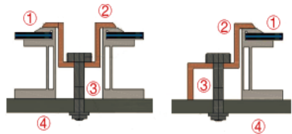
frame clip M8 bolt mounting rail
